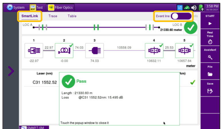
Figure 9: SmartLink View, Summary Results
