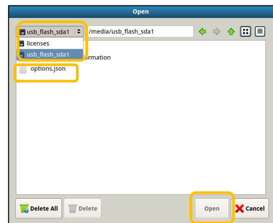
Figure 6: Import Options
