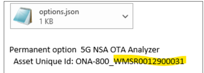
Figure 4: Options file
