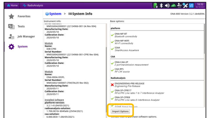
Figure 5: System Info
