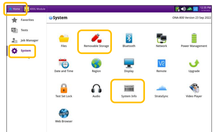
Figure 2: System Menu
