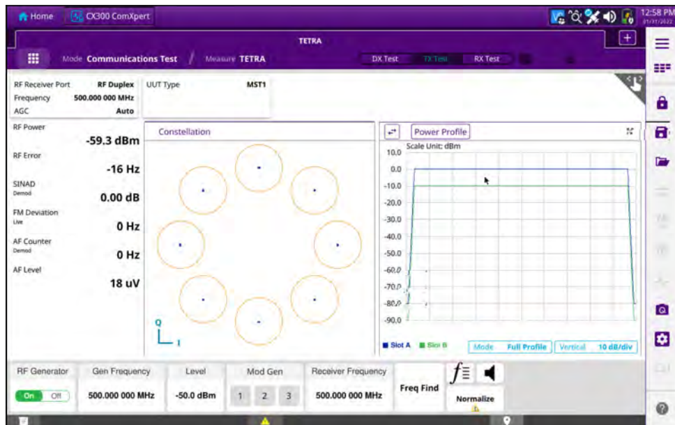
Figure 1-4 TETRA User Interface (UI) - Example only
